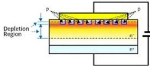
Junction Barrier SBD structure
